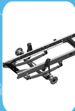
First in Class Parabolic Suspension
